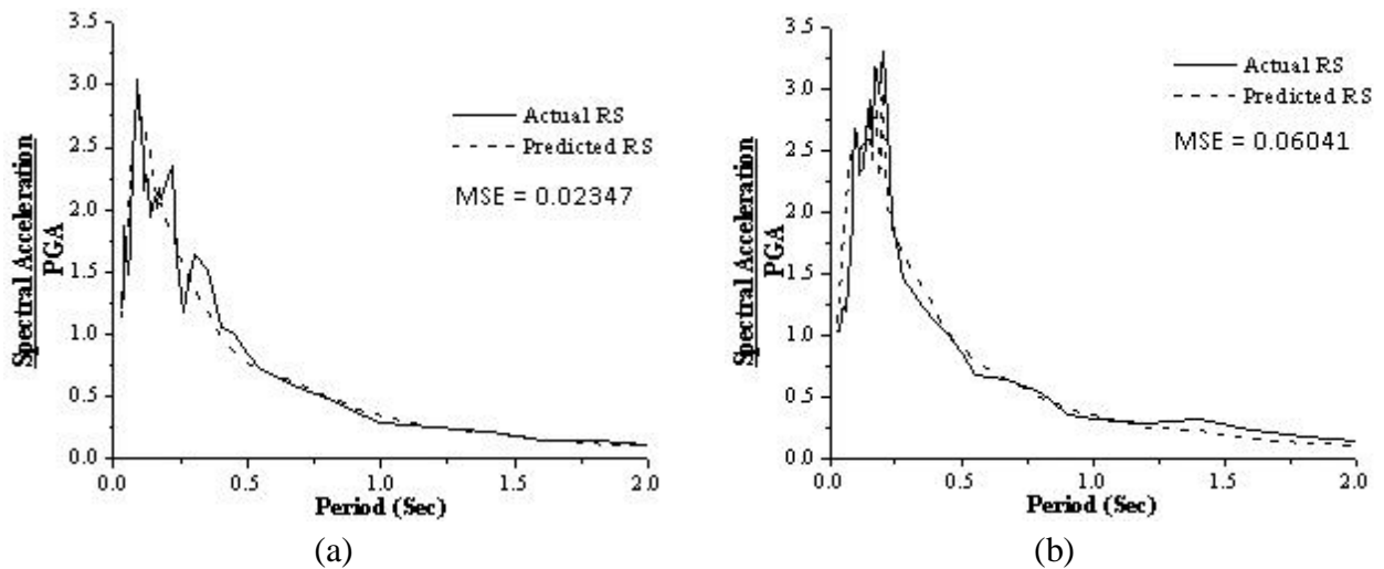
Fig. 8 Typical plots of acceleration response spectra predicted by ANN with three inputs for (a) M = 5.2 , H = 42 km, \bar{v}_s = 455.5 m/s and (b) M = 5.1 , H = 39.6 km, \bar{v}_s = 345.8 m/s
