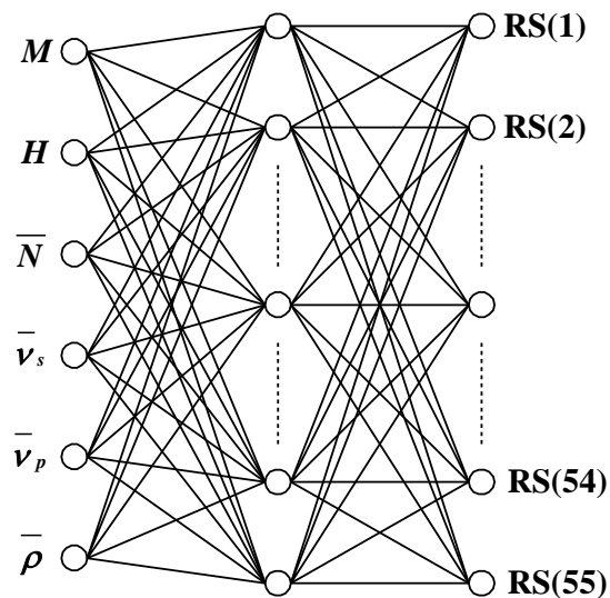
Fig. 6 Neural network architecture with six inputs
