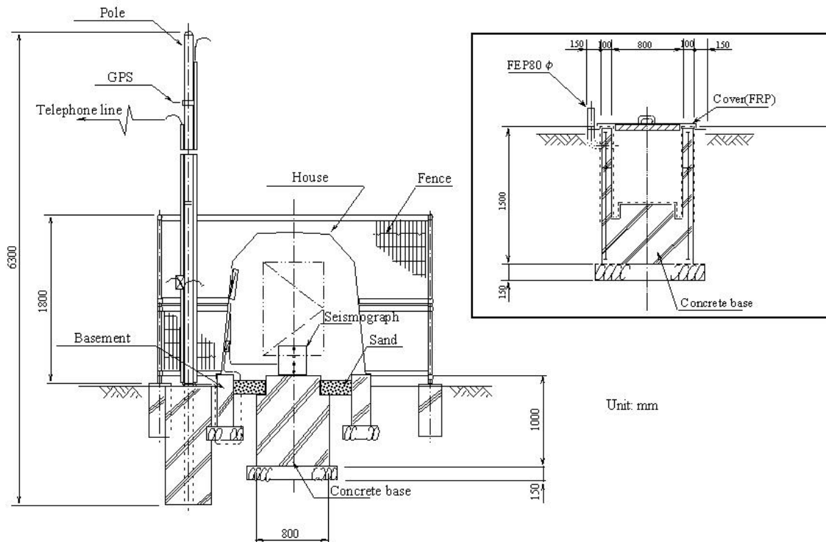
Fig. 1 The layout of typical observatory 1
