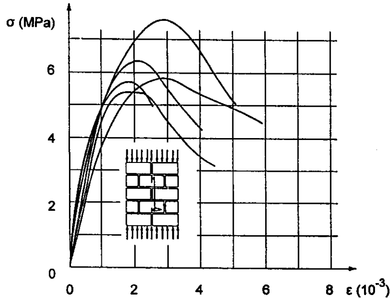
Fig. 2 Typical experimental stress-strain relationship of masonry at compression (Tomažević and Žarnić, 1984)
