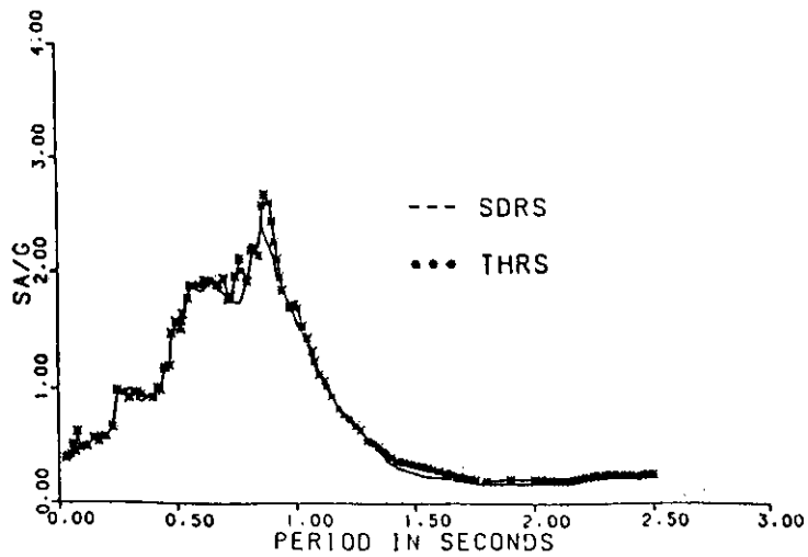
Fig. 4 HORI. ACCL. SPEC. SAMPLE (N-S)
