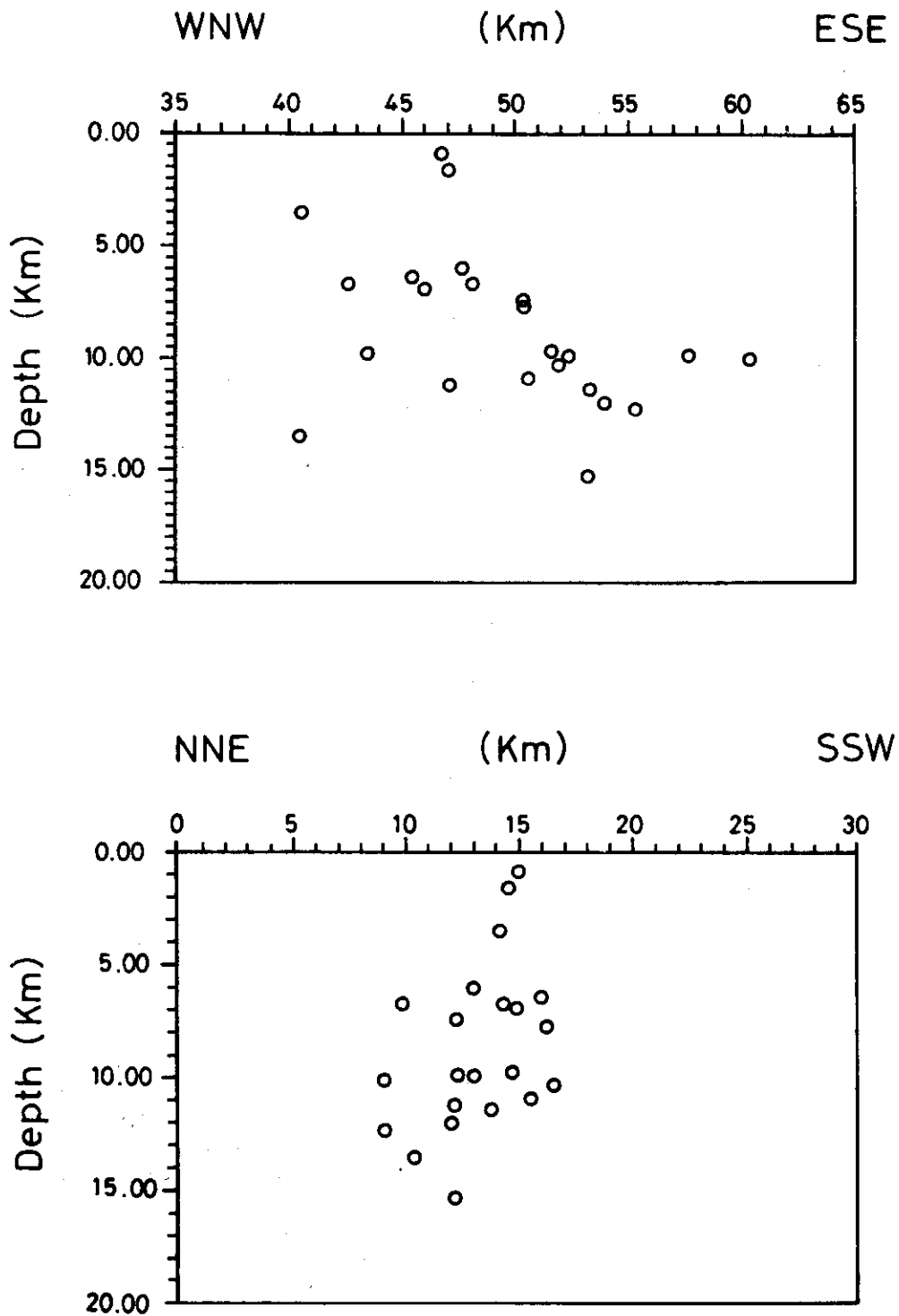
Fig. 4 Depth sections (a) along and (b) transverse to the strike of the epicentral belt.
