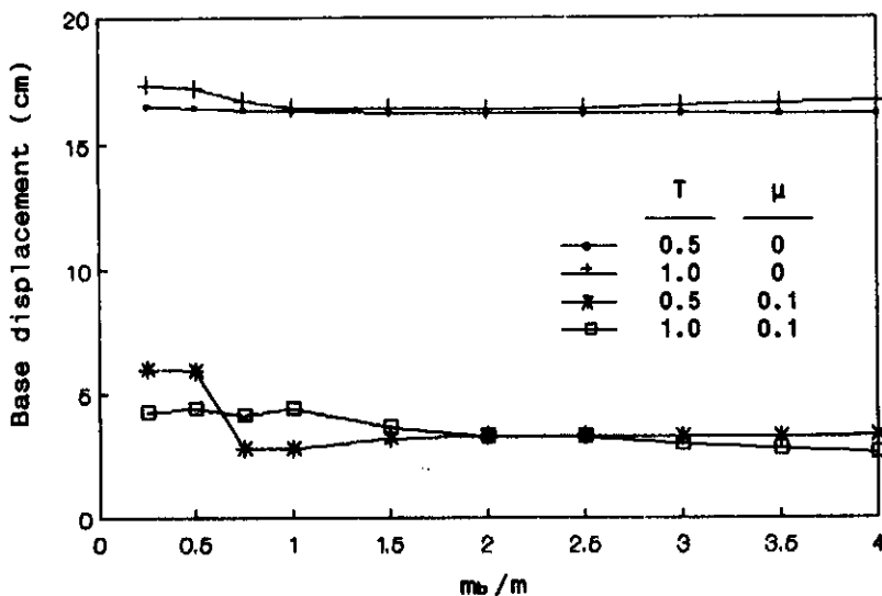
Fig. 9 Variation base displacement against mass ratio m_b/m . for T_b = 2 sec and \%_b = 0.1
