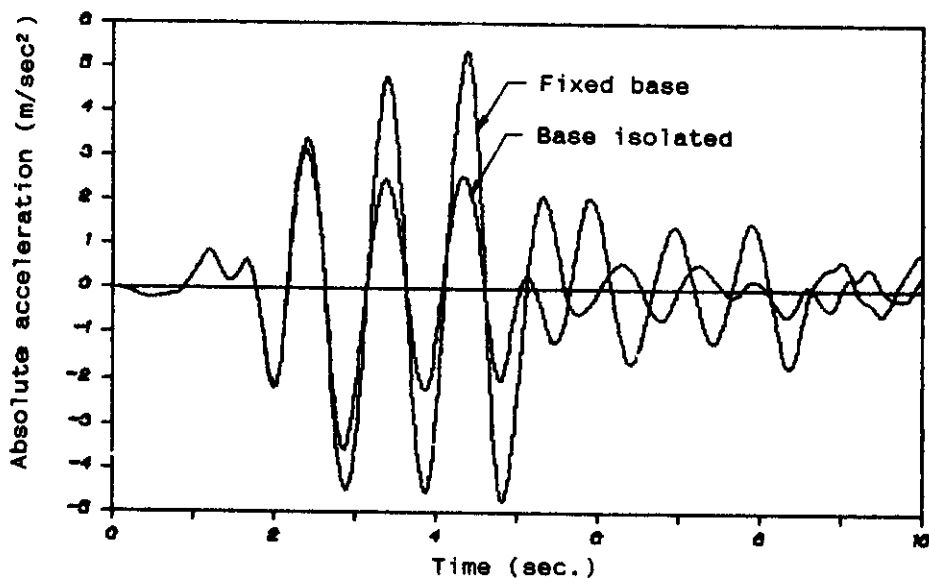
Fig. 4 Time variation of absolute acceleration of the deck: T = 1 sec., m_b/m = 1.5 , T_b = 2 sec., \mu = 0.1 and \xi_b = 0.1
