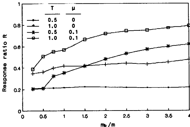
Fig. 8 Plot of response ratio R against mass ratio m_b/m . for T_b = 2 sec and \%_b = 0.1
