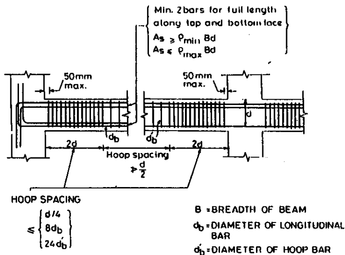
Fig. 5 BEAM REINFORCEMENT
