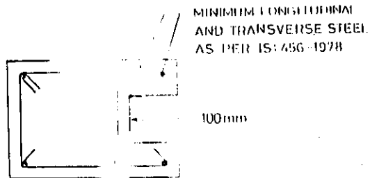
Fig. 7 REINFORCEMENT REQUIREMENT FOR COLUMN WITH MORE THAN 100 mm PROJECTION BEYOND CORE
