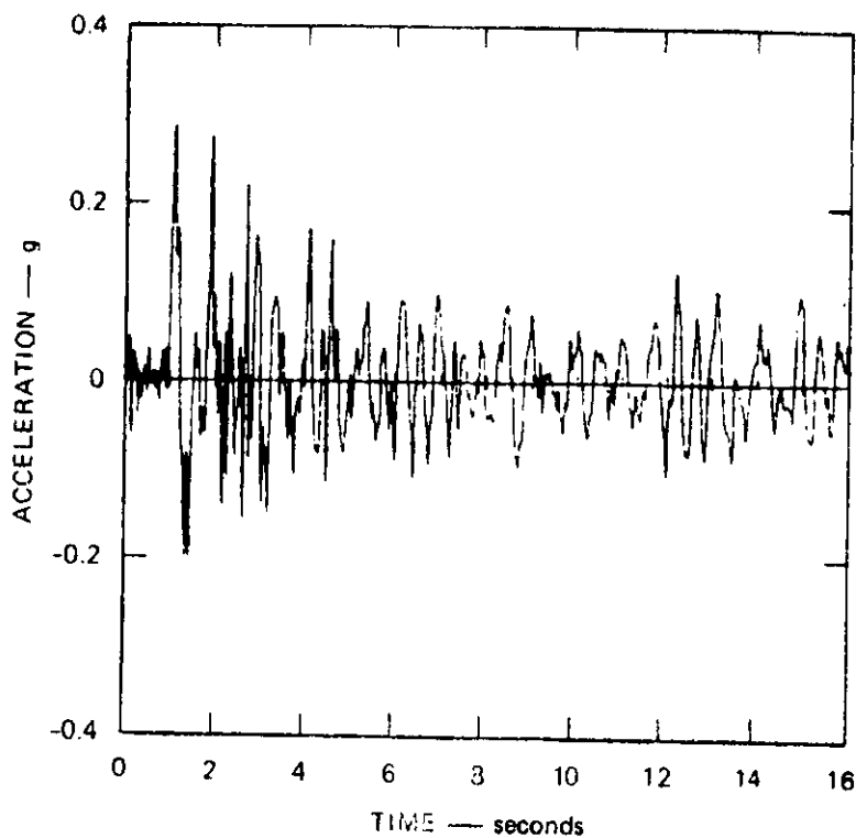
Fig. 1. Accelerogram for San Fernando, California Earthquake (February 9, 1971, Castaic N 69 W)
