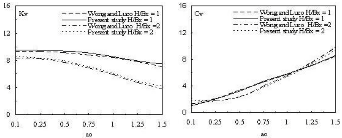
Fig. 6 Validation of vertical impedance function of square rigid foundation resting on layer overlying semi-infinite soil for varying relative ratio of layer thickness ( H/B_x = 1, 2 ), with C_{s1}/C_{s2} = 0.8 and \rho_2/\rho_1 = 1.13 (uniform layer case)
