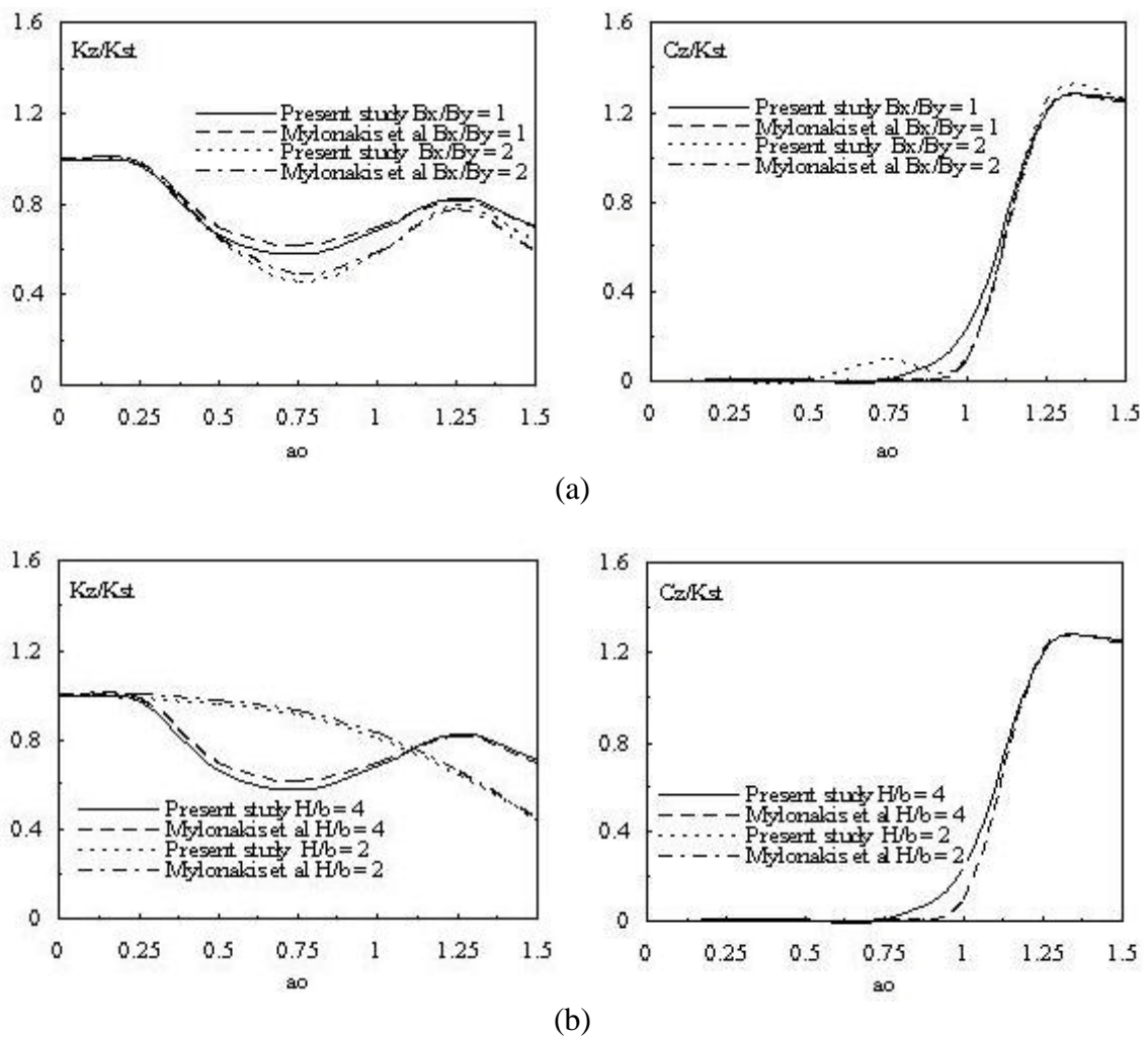
Fig. 7 Validation of vertical impedance function of rigid foundation on soil layer over bedrock: (a) rectangular surface foundation for varying relative length, with H/B_x = 4 ; (b) square surface foundation for varying depths of the substratum
