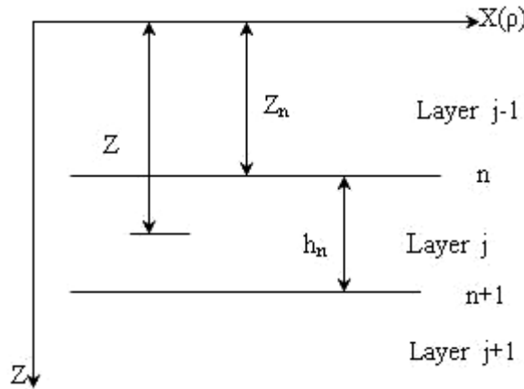
Fig. 3 Geometry of layered stratum B
