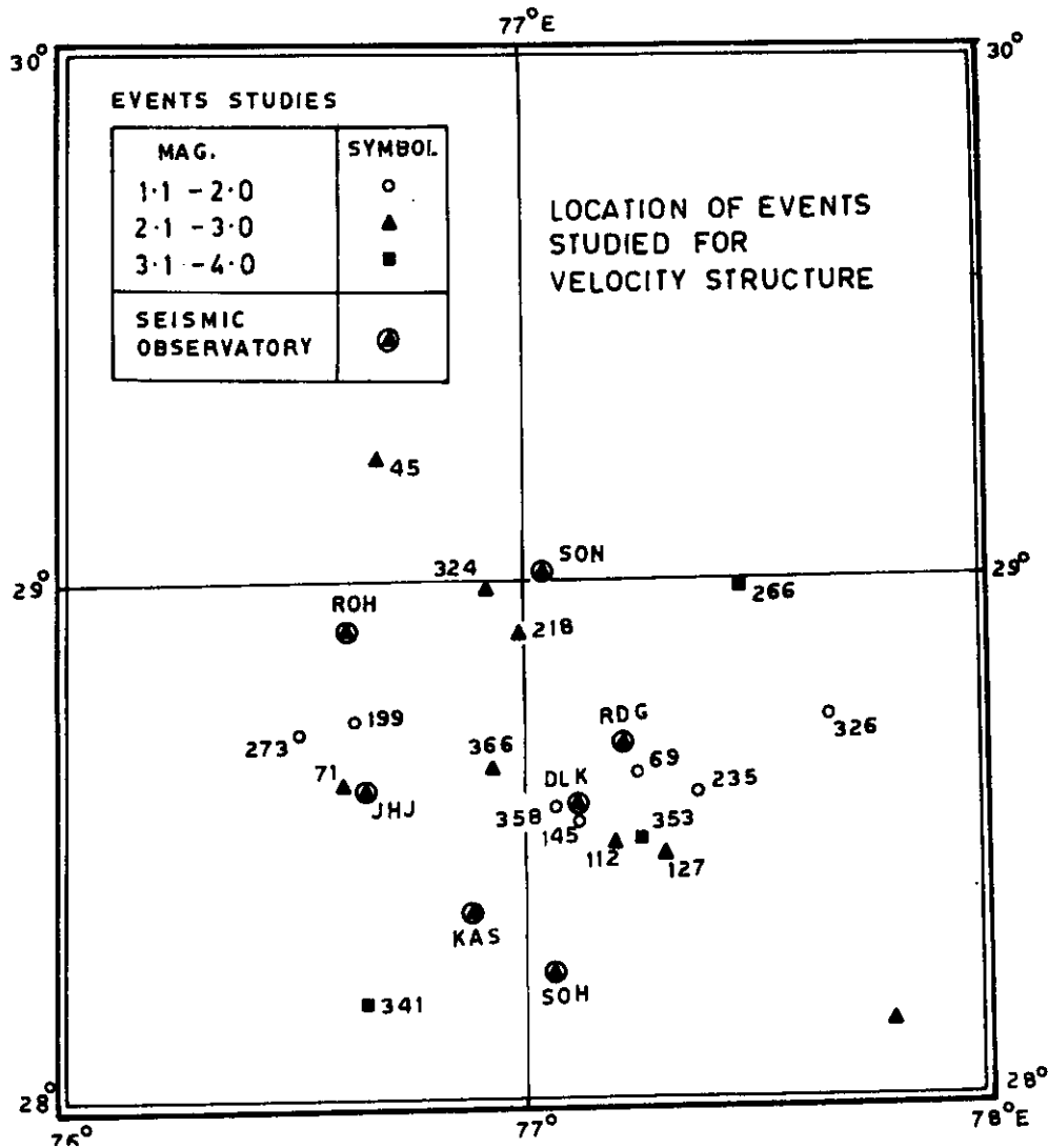
Fig.2 Locations of the events used in the analysis of Pg and Sg wave velocities are shown alongwith the recording stations. Abbreviations : ROH-Rohtak, SON-Sonepat, RDG-Ridge, SOH-Sohna (IMD network), JHI-Jhajjar, DLK-Daula Kuan and KAS-Kasan.
