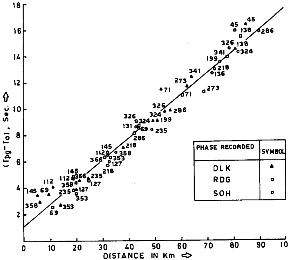
Fig. 4 A plot of (T_{pg}-T_o) vs epicentral distance (km) for the sta used. The inverse of slope of least square fit gives the Pg wave velocity of 6.06 \pm 0.12 km/sec.
