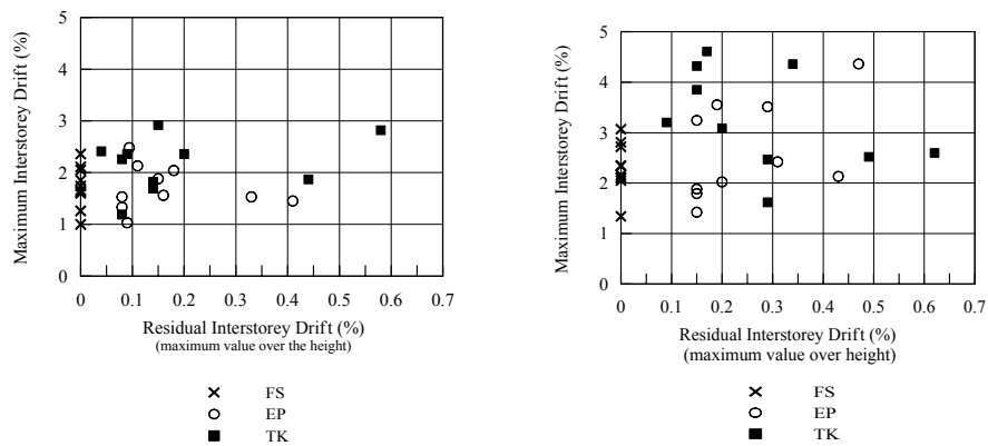
Fig. 10 New-designed frame systems response (without P-\Delta effects) at BSE-1 (left side) and BSE-2 (right side) levels: RD-based performance matrix
