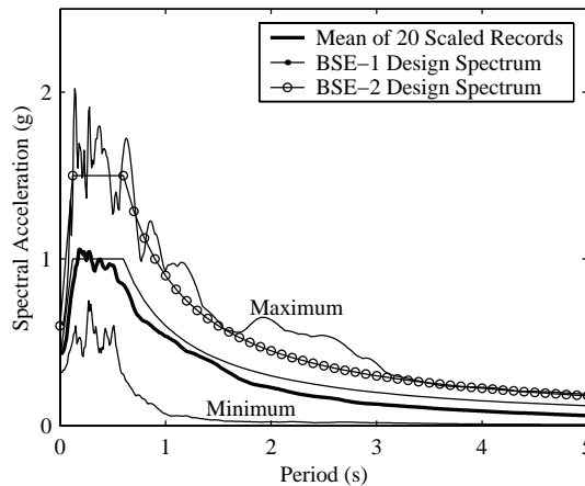
Fig. 5 Elastic acceleration response spectra (5% elastic damping) of the considered ground motions
