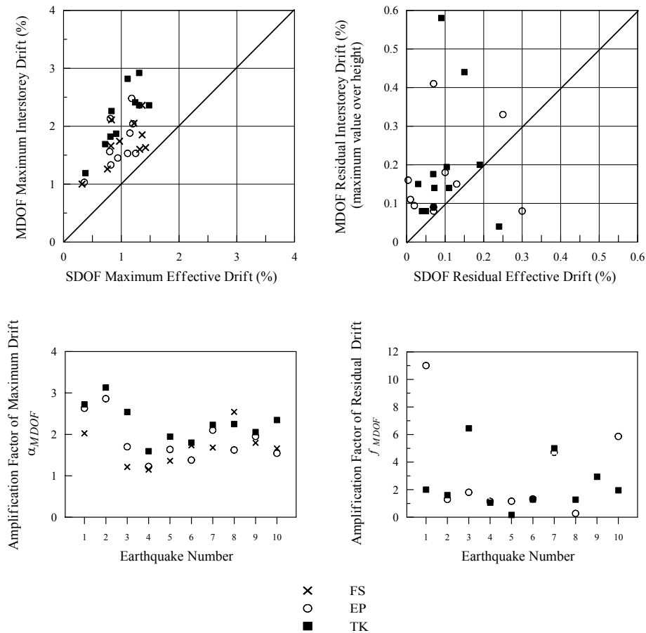
Fig. 11 New-designed frame systems response at BSE-1 level (without P-\Delta effects): Maximum drift and residual drift amplification factors due to higher modes
