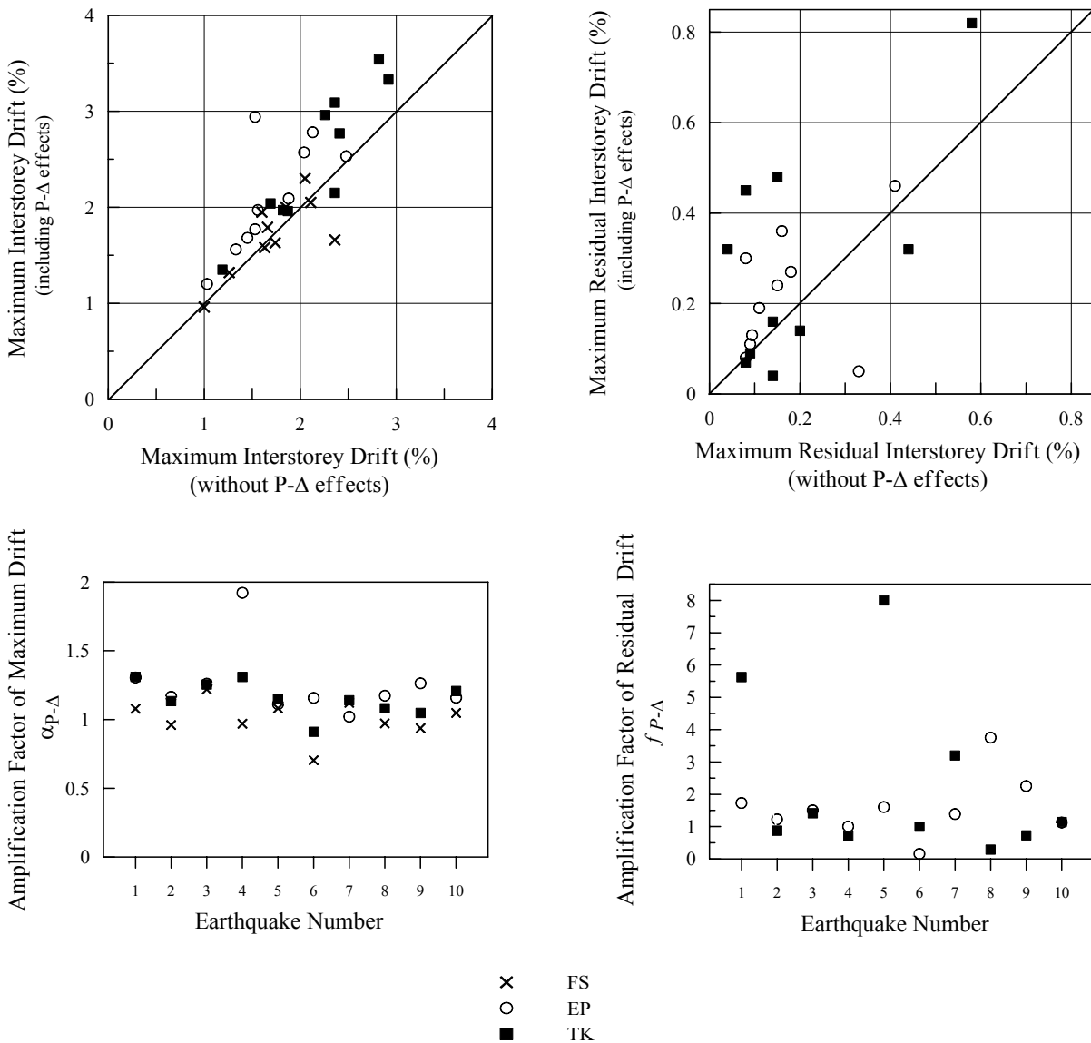
Fig. 12 New-designed frame systems response at BSE-1 level: Maximum drift and residual drift amplification factors due to P-\Delta effects
