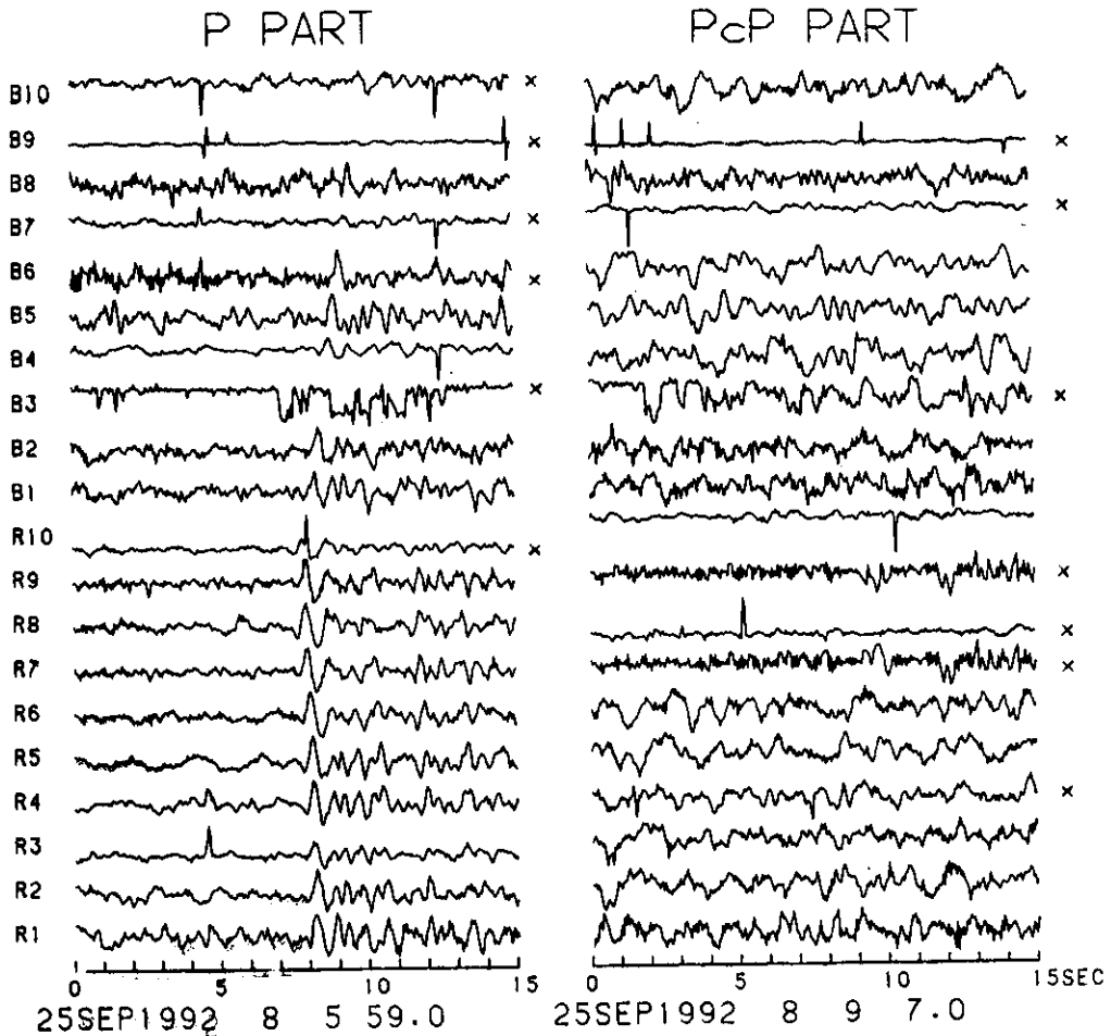
Fig. 1: Raw (unprocessed) waveforms plotted from digital data obtained at GBA corresponding to P and PcP parts (PcP signal is not discernible) of the recent Chinese underground nuclear explosion (magnitude Mb 5.0; yield approximately 15kt) at Lop Nor, Southern Xinjiang Province, on 25 September 1992. Labeled from R1 to R10 and B1 to B10 corresponding to twenty channels of the seismic array, each of the waveforms is reproduced for 15 seconds starting from 08:05:59.0 and 08:09:07.0 GMT respectively as shown by 1 sec time marks at bottom. Unsatisfactory recordings in some channels marked by crosses (x) are not used in further processing.
