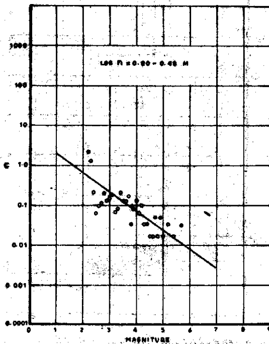
Fig. 8b. Mean Annual Frequency Distribution of Earthquakes in Alesund-Stavanger Seismotectonic Belt (1891-1950)
