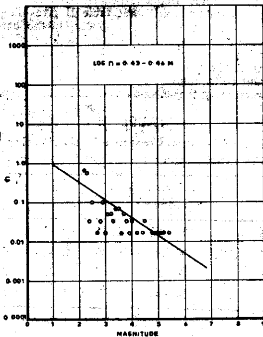
Fig. 8c. Mean Annual Frequency Distribution of Earthquakes in Alesund-Tromso Seismotectonic Belt (1891-1950)
