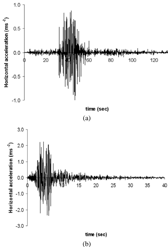
Fig. 1 Strong motion records for the Bhuj and Uttarkashi earthquakes: (a) Bhuj earthquake record at Ahmedabad; (b) Uttarkashi earthquake record at Uttarkashi
