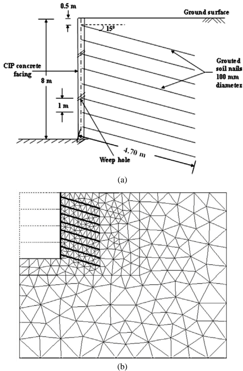
Fig. 2 Soil nail wall supporting the 8-m high vertical cut: (a) outline of the designed soil nail wall; (b) the numerically modelled state
