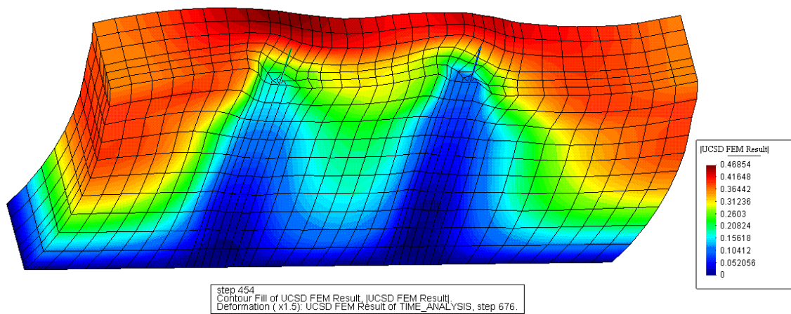
Fig. 11 Sketch of deformed mesh (factor of 1.5; color map shows longitudinal displacement in meters) at 10 s (He, 2005), clearly showing significant reduction in lateral displacement around the piles (the pile-pinning effect)
