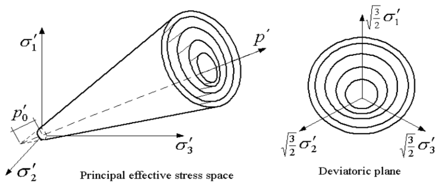
Fig. 1 Conical yield surfaces for granular soils in principal stress space and deviatoric plane (after Prevost, 1985; Yang et al., 2003)
