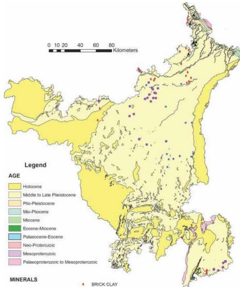
Fig. 4 Geomorphological Map of Haryana (GSI, 1973)
