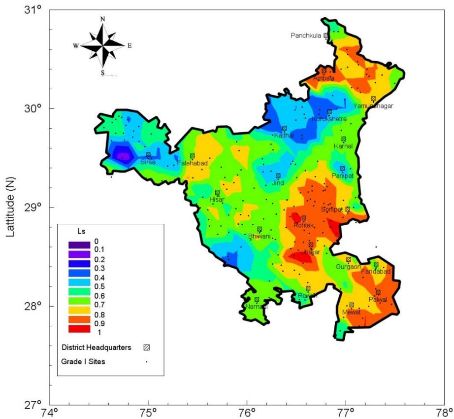
Fig. 6 Grade-I Liquefaction Susceptibility Map
