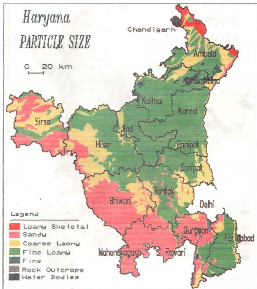
Fig. 3 Soil Resource Map (Sachdev et al., 1995)
