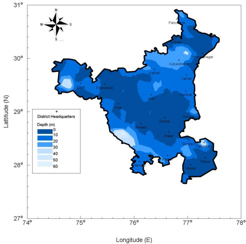
Fig. 5 Water Table Map
