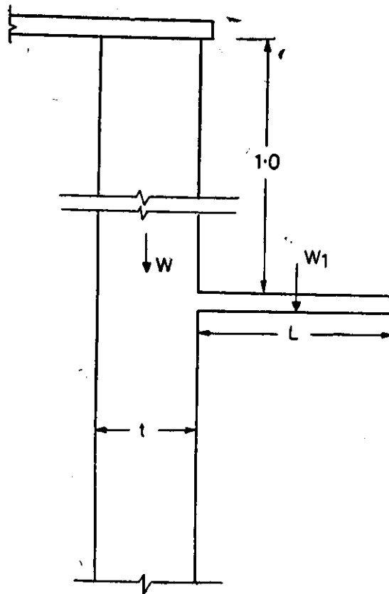
Fig. 2 Schematics of the Horizontal Cantilever
