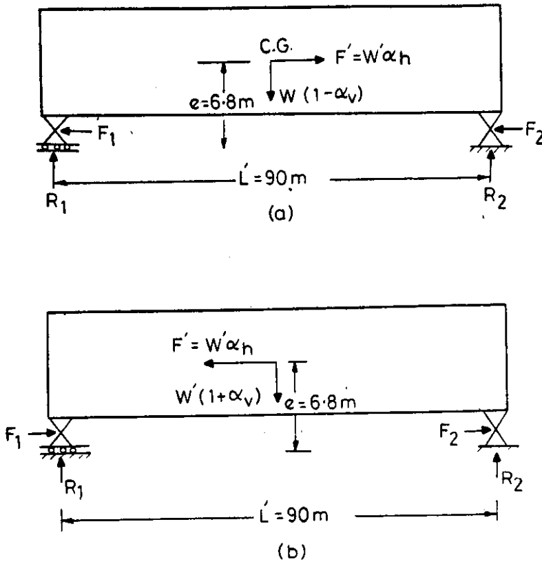
Fig. 3 Schematics of Forces Acting on the Bridge
