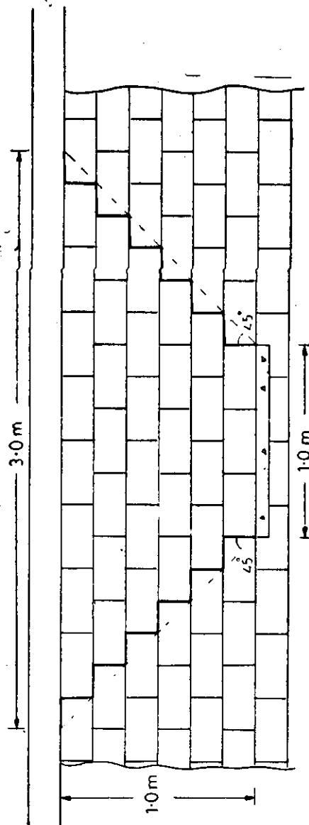
Fig. 1 Assumed Failure Line due to Overturning
