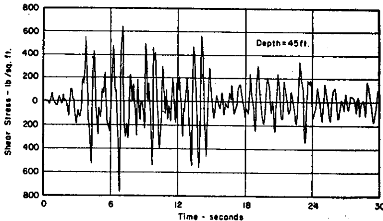
Fig. 2. Cyclic Shear Stress on a Soil Element during Ground Shaking
