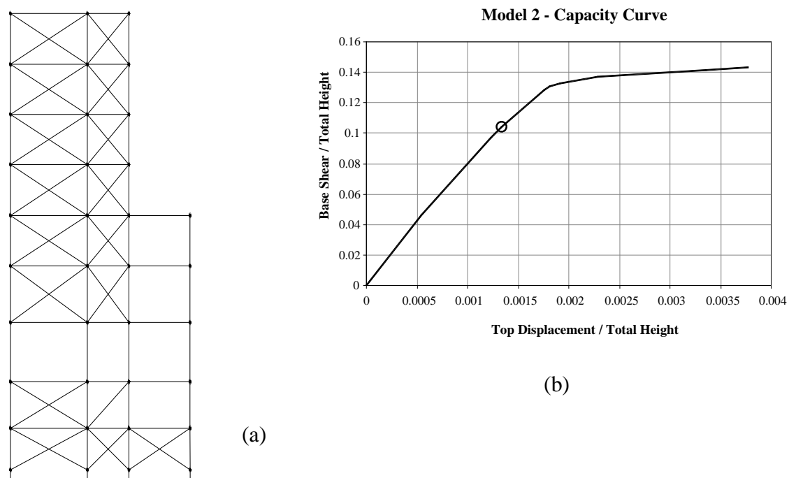
Fig. 9 Model 2 – (a) Removal of collapsed masonry struts; (b) Capacity curve based on first mode (for Model 2)
