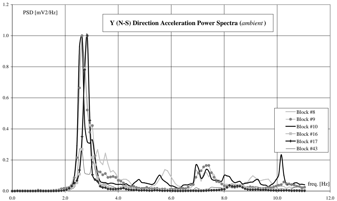
Fig. 3 Normalized ambient vibration acceleration power spectrum for building blocks #8, 9, 10, 16, 17 and 43 (Y - N-S direction)
