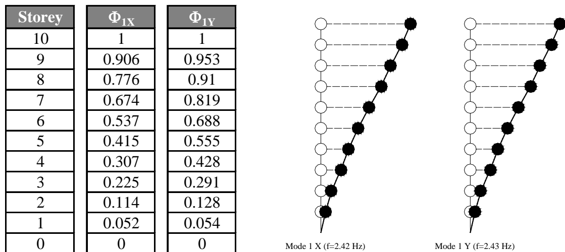
Fig. 4 Fundamental mode shapes for building block #4 (X - E-W direction, Y - N-S direction)
