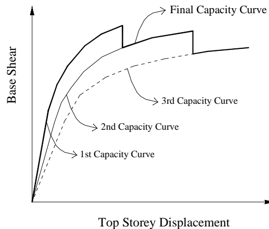
Fig. 8 ATC pushover curve, obtained from several capacity curves, as indicated in (Applied Technology Council, 1996)
