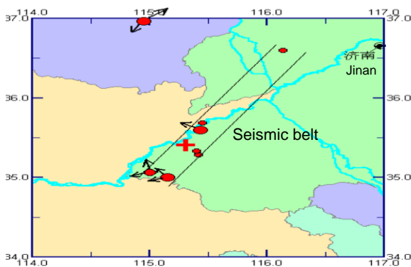
Fig. 10 Primary rupture directions of small and medium earthquakes that occurred on the seismic belt before the Heze M 5.9 earthquake
